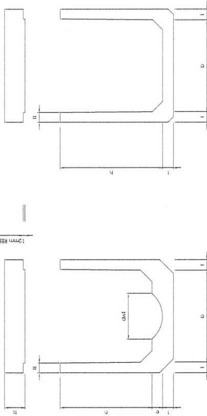
Box Culvert c/w DWF
